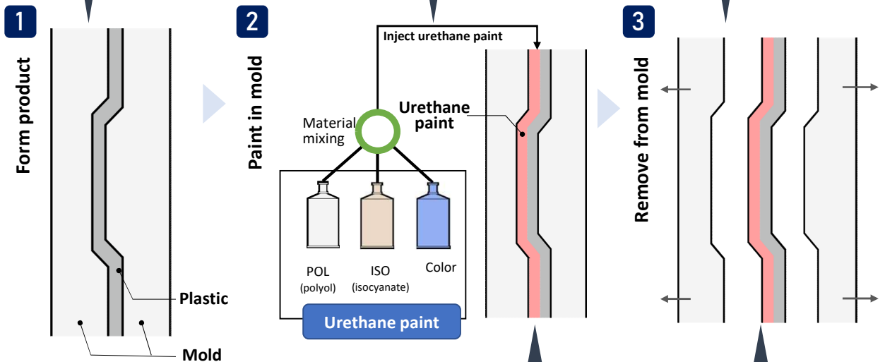
POINT 4 Fluidity of paint (spreadability)
